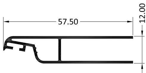
5234 LAMA TERMINAL
